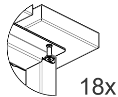
DETAIL 4
